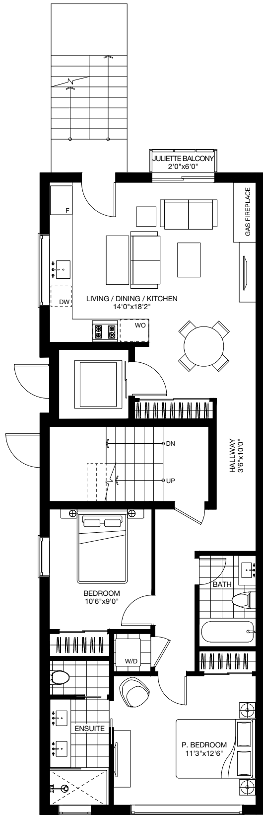
MAIN LEVEL
